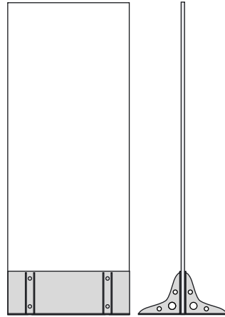
zeta 218 w 700 x h 1800 x d 500mm w 27,56 x h 70,87 x d 19,69"
