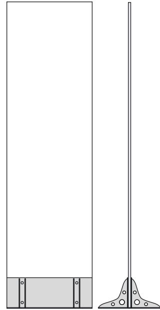
zeta 225 w 700 x h 2500 x d 500mm w 27,56 x h 98,43 x d 19,69"
