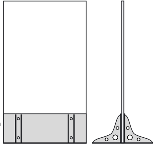
zeta 212 w 700 x h 1200 x d 500mm w 27,56 x h 47,24 x d 19,69"
